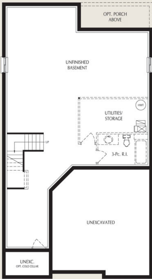
BASEMENT PLAN
