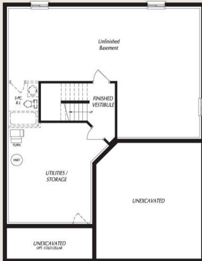
BASEMENT PLAN
