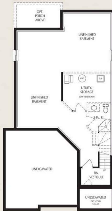
BASEMENT PLAN WITH SUNKEN FORMAL ROOM
